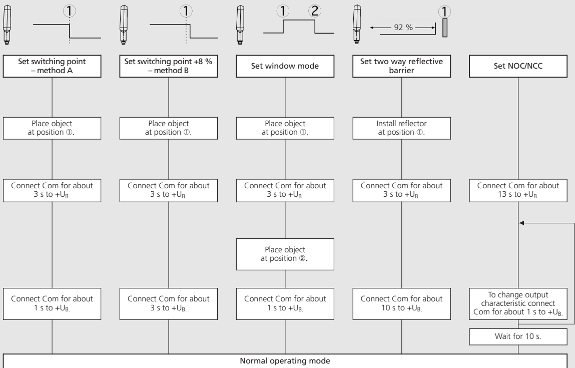
Teach-in switching output
