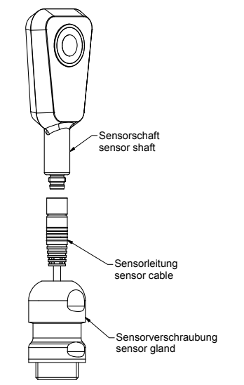
Fig. 4: Mounting of pms sensor with sensor screw connection BF-pms/A1
