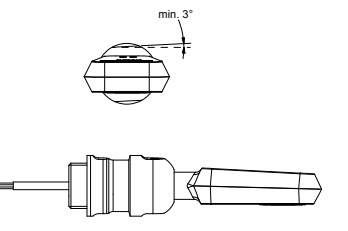
Fig. 3: pms sensor D12-adapter shaft with sensor screw connection BF-pms/A1, all surfaces must be inclined at least 3°.
