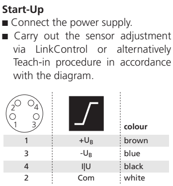
Fig. 1: Pin assignment with view onto sensor plug and colour coding of the microsonic connection cable
