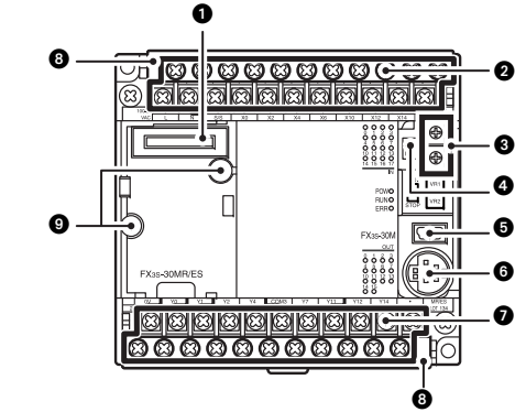
View with covers removed
