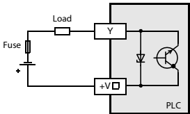
Transistor output (source)
