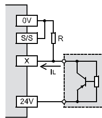
PNP (source)
