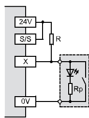
NPN (sink)
