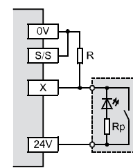
PNP (source)
