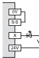
Circuito a logica positiva PNP (Source)
