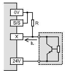
Circuito a logica positiva PNP (Source)
