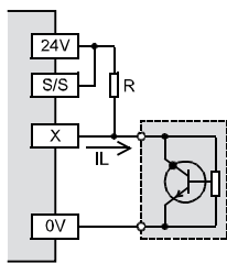
NPN (sink)
