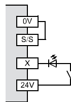
PNP (source)
