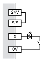
NPN (sink)
