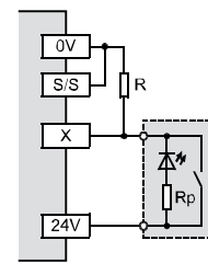
Circuito a logica positiva PNP (Source)
