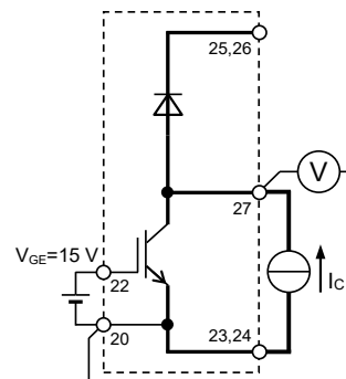
Brake IGBT
