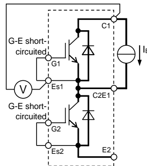
V_{EC} characteristics test circuit
