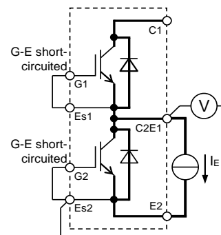
V_{EC} characteristics test circuit
