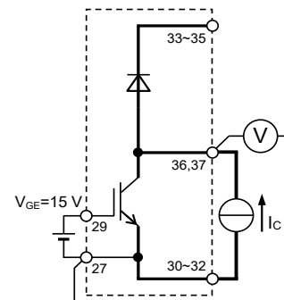
Brake IGBT
