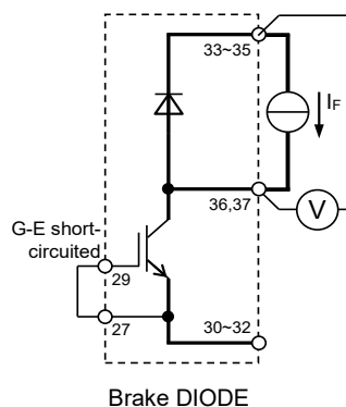
Brake DIODE
