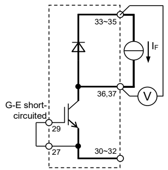
Brake DIODE
