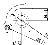
MOUNTING HOLES
