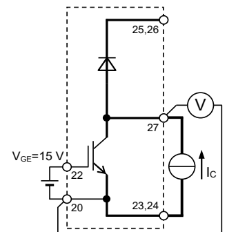
Brake IGBT
