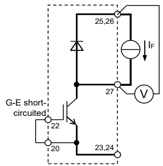
Brake DIODE
