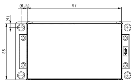
PCB DRILL HOLE PATTERN
