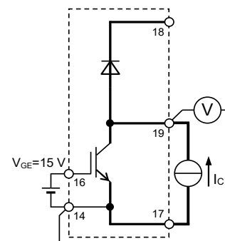
Brake IGBT
