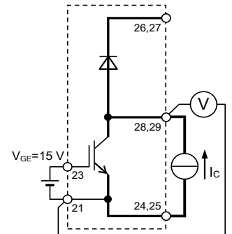
Brake IGBT
