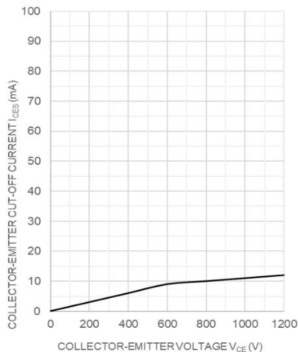
COLLECTOR-EMITTER CUT-OFF CURRENT CHARACTERISTICS (TYPICAL)
