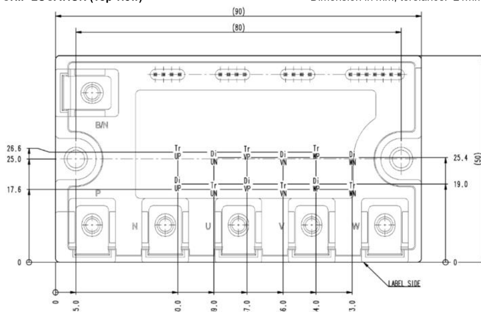
CHIP LOCATION (Top view)
