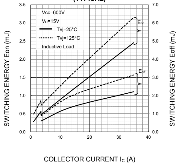
SWITCHING ENERGY CHARACTERISTICS (TYPICAL)
