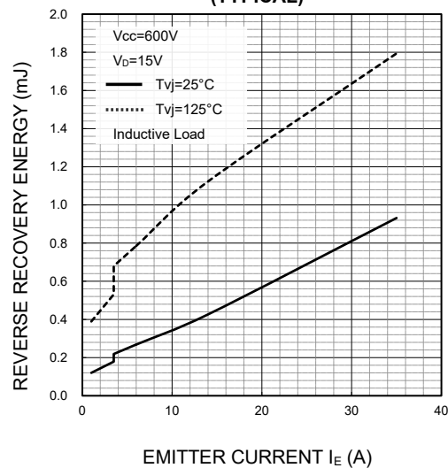
FREE WHEELING DIODE REVERSE RECOVERY ENERGY CHARACTERISTICS (TYPICAL)
