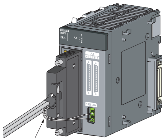
Wiring to the differential driver common terminal
