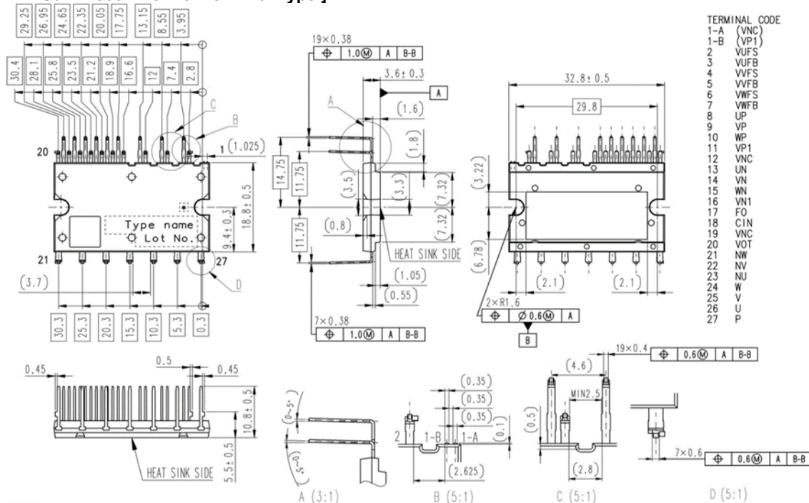
Fig. 11 Package Outlines
