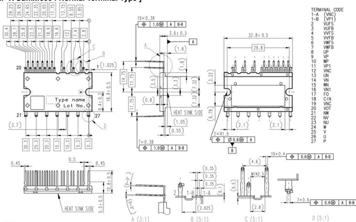
Fig. 11 Package Outlines
