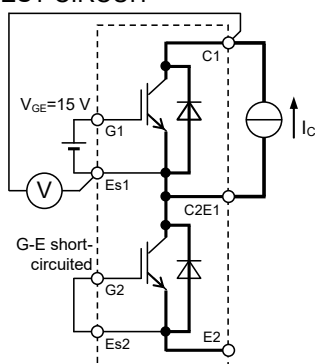
V_{CEsat} characteristics test circuit
