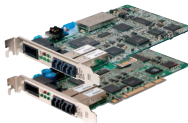
Q81BD-J71GP21S-SX/ Q80BD-J71GP21S-SX External power supply I/P terminal type
