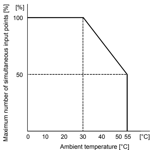
(b) Dilating curve for the AJ65MBTL1N-32D
