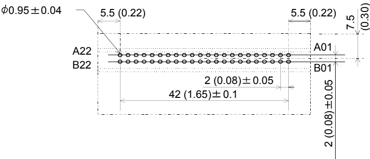
[Recommended board dimension drawing] (top view)
