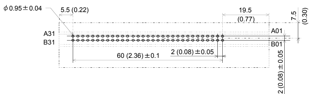
[Recommended board dimension drawing] (top view)
