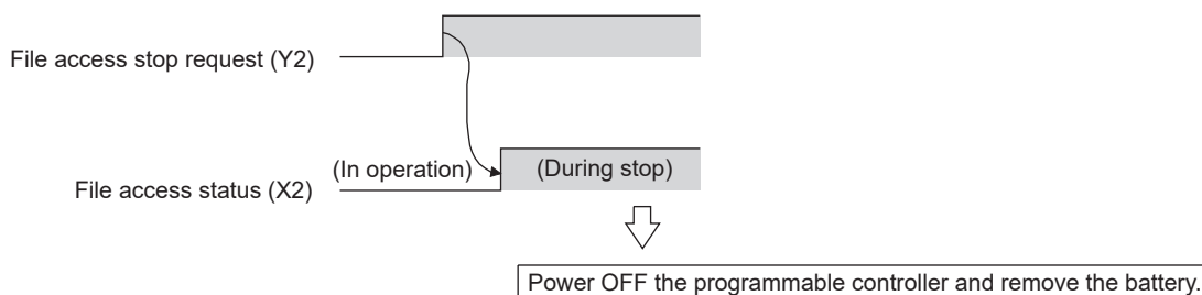
Figure 4.19 Removing battery for storage
