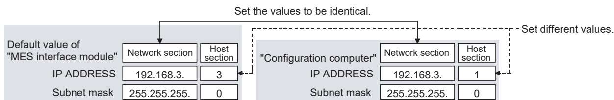
Figure 2.5 Network settings for configuration computer
