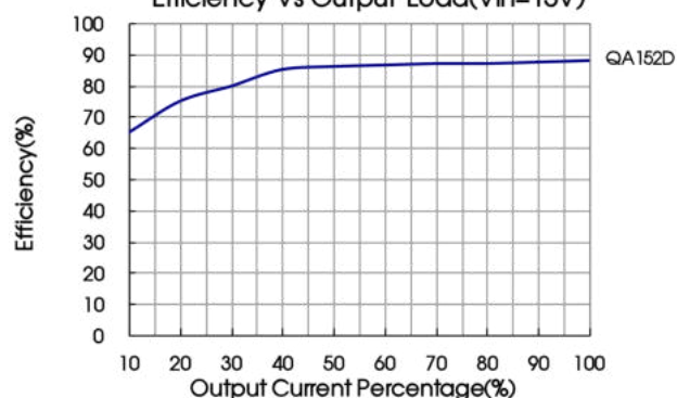
Efficiency Vs Output Load(Vin=15V)
