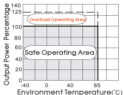
Operating Temperature Curve
