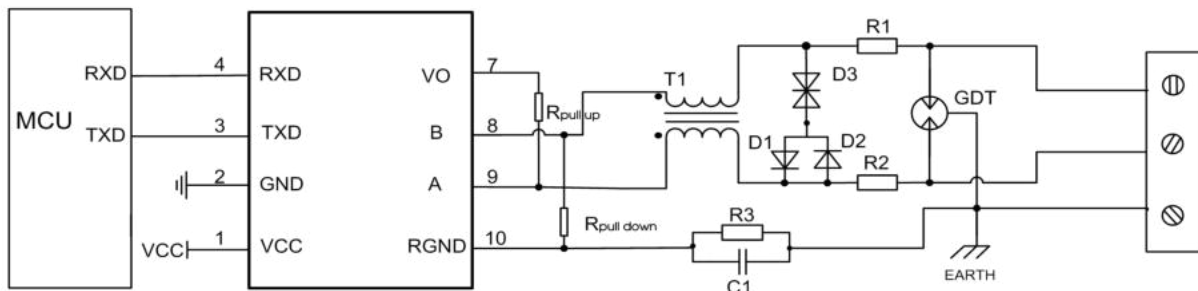
Fig. 2: Port protection circuit for harsh environments
