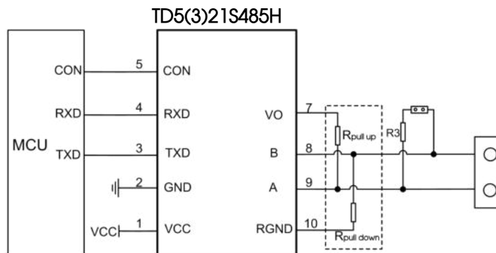
Fig. 1: Typical application
