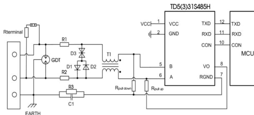
Fig. 2: Port protection circuit for harsh environments
