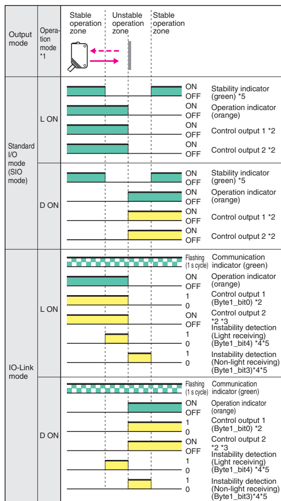
Timing Chart
