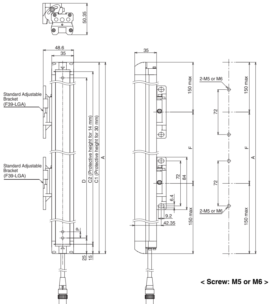
F3SG-4RE□□□□30 Series
