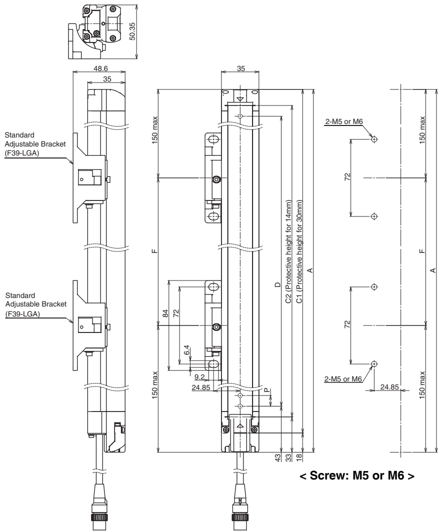
F3SG-□RA□□□□-30 Series
