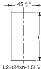
Vertically Group Mounted
