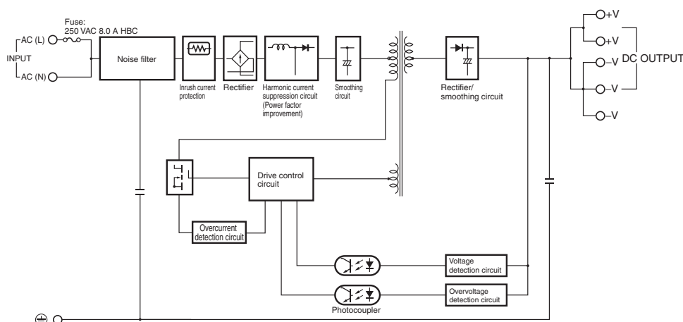
S8VK-C24024 (240W)
