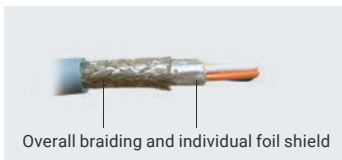
Shield structure
