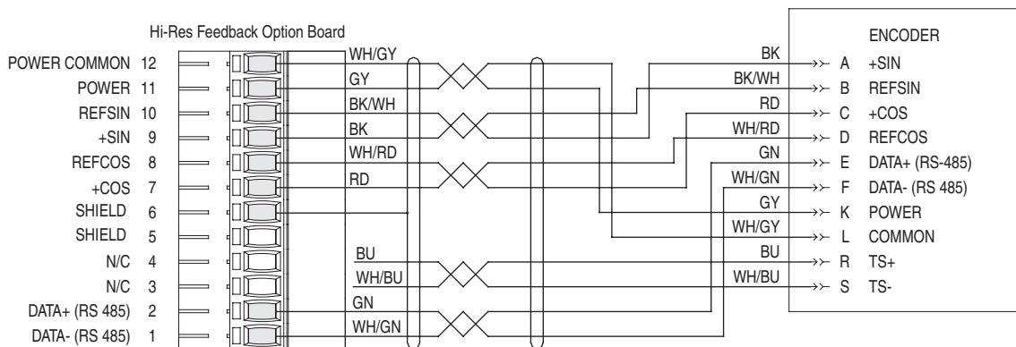
Figure E.5 Stegmann shielded twisted-pair cable with 12-pin DIN style connector
