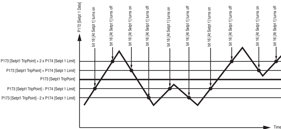
Figure C.5 At Setpoint 1 Status
