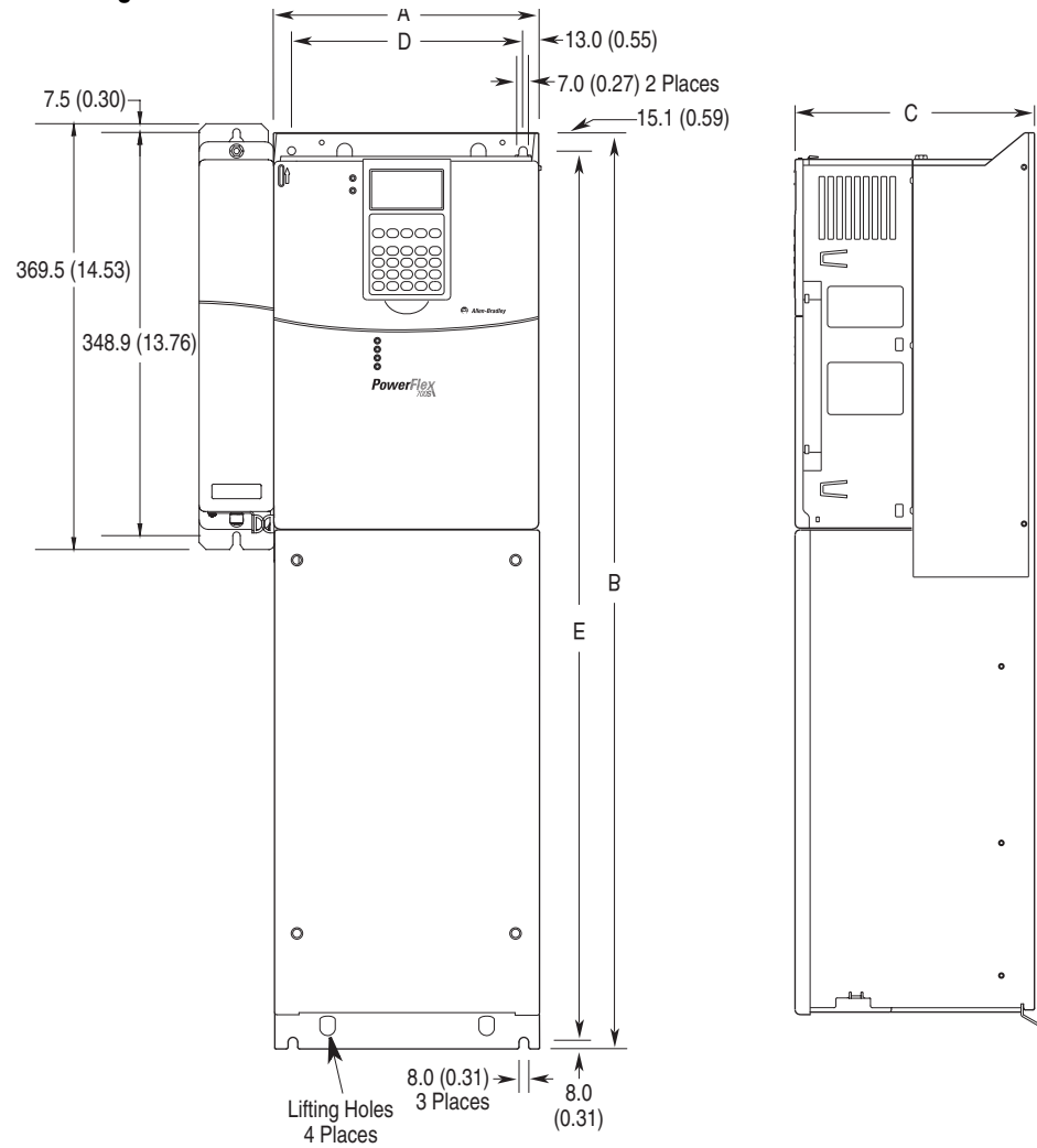
Figure A.2 PowerFlex 700S Frame 4
