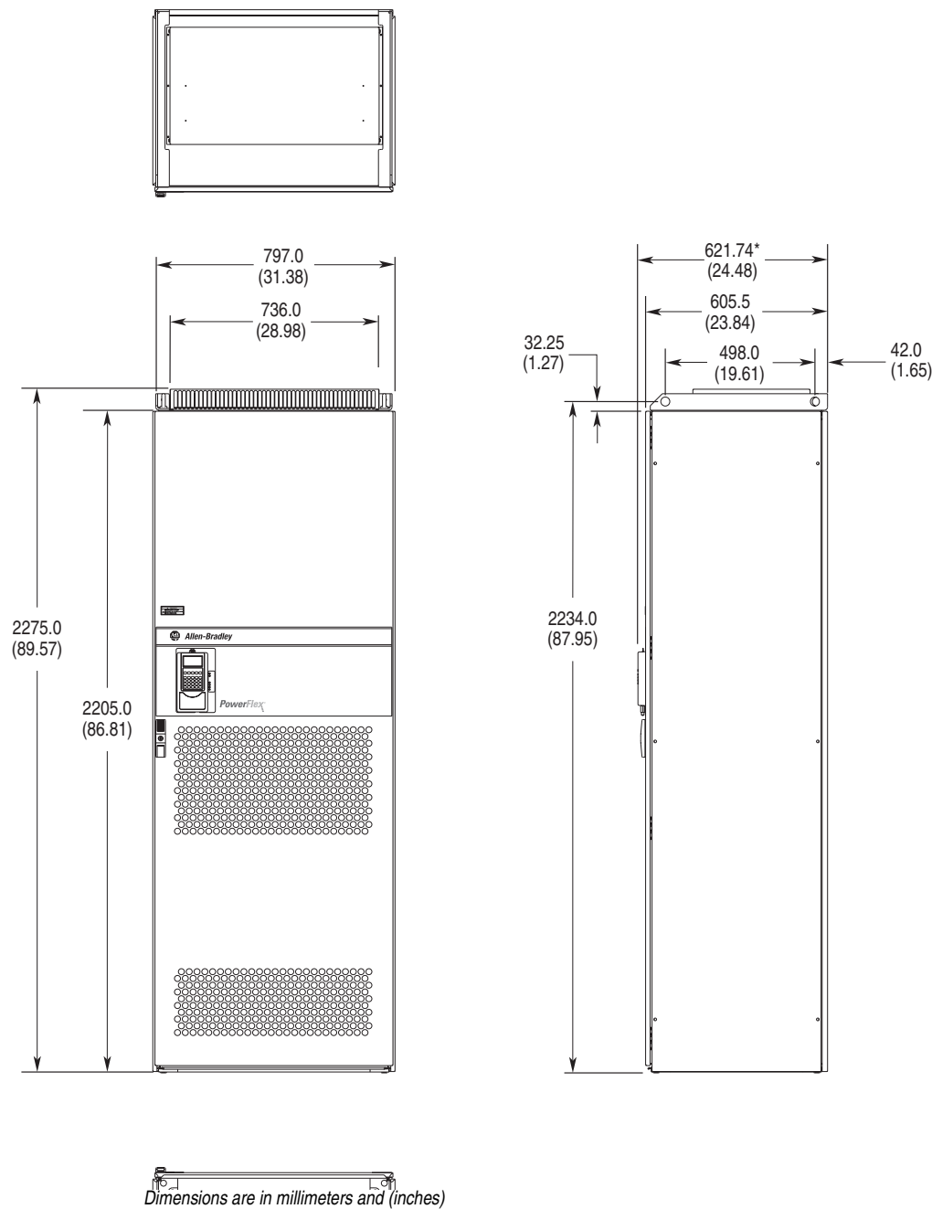
Figure A.7 PowerFlex 700S Frame 11
