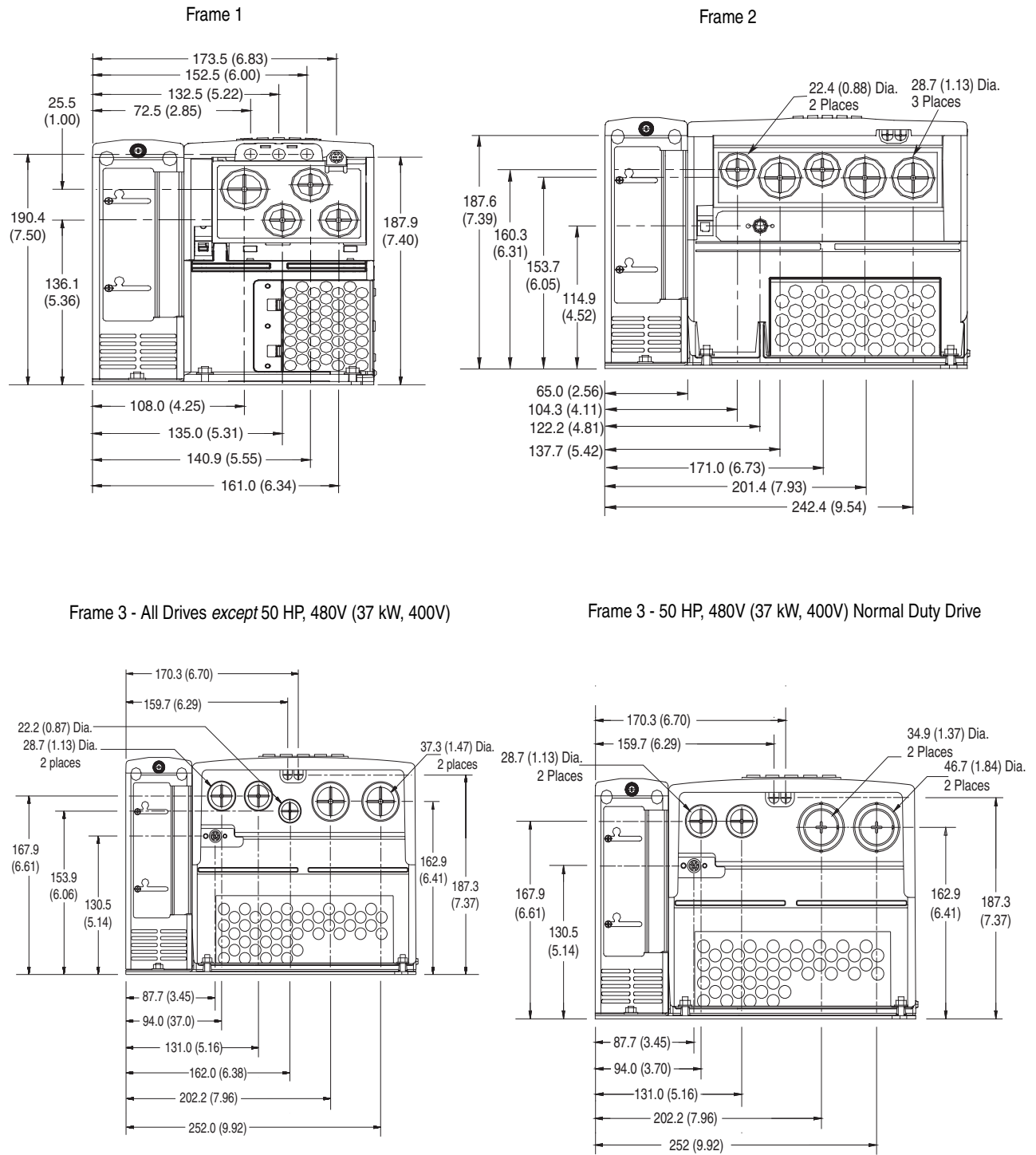
Figure A.8 PowerFlex 700S Bottom View Dimensions
