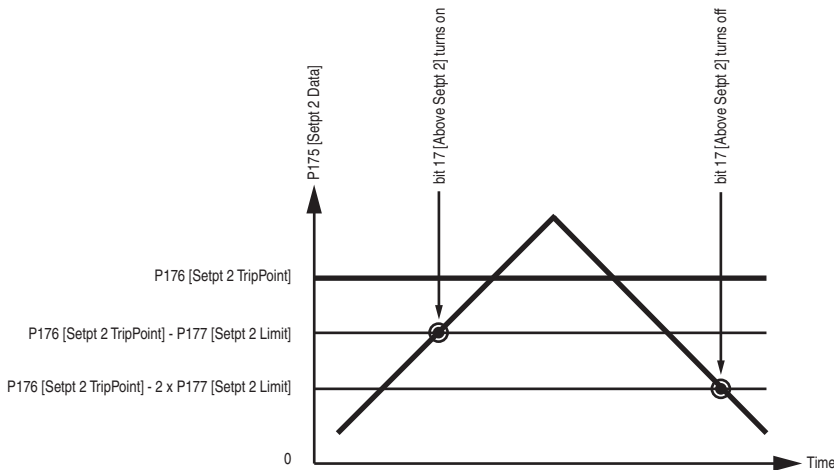
Figure C.6 Above Setpoint 2 Status
