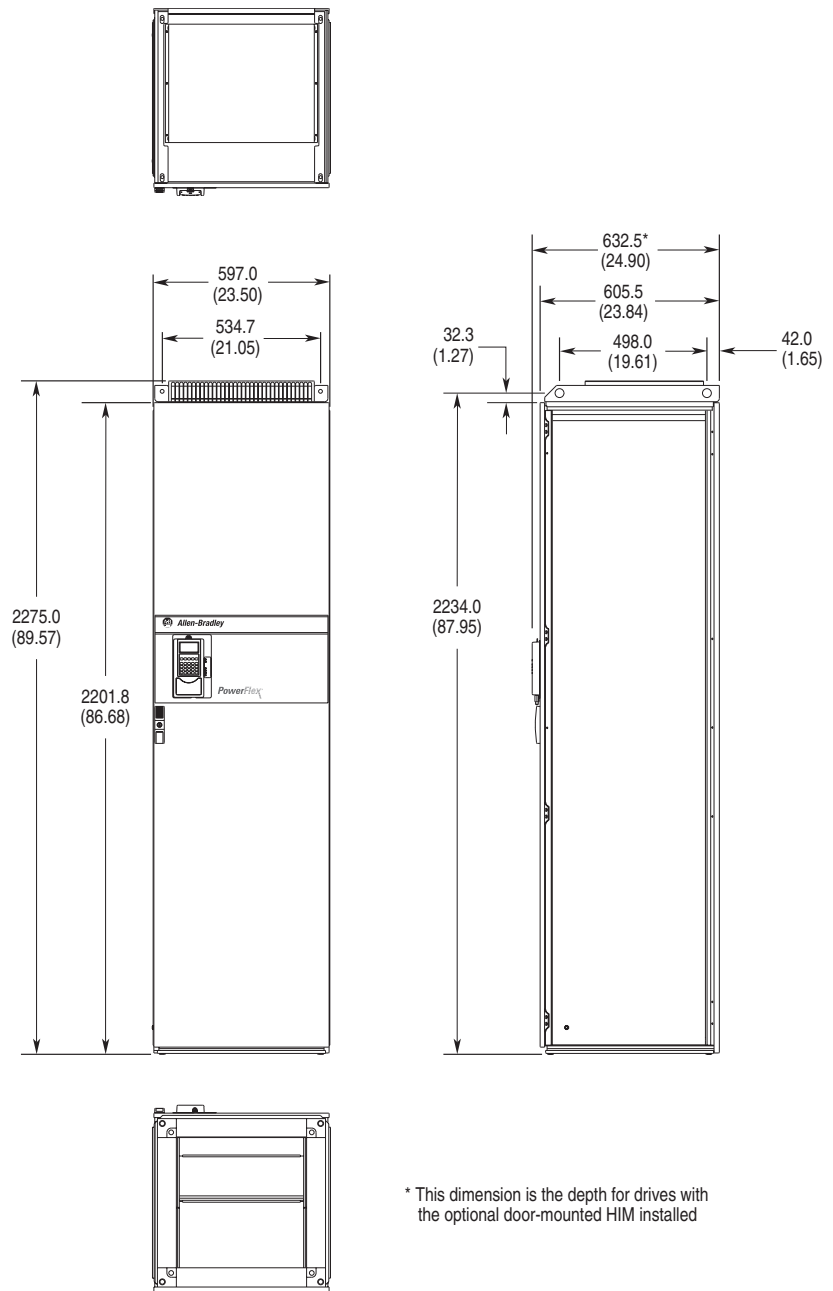
Figure A.6 PowerFlex 700S Frame 10
