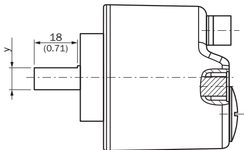
Dimensional drawing Solid shaft, face mount flange
