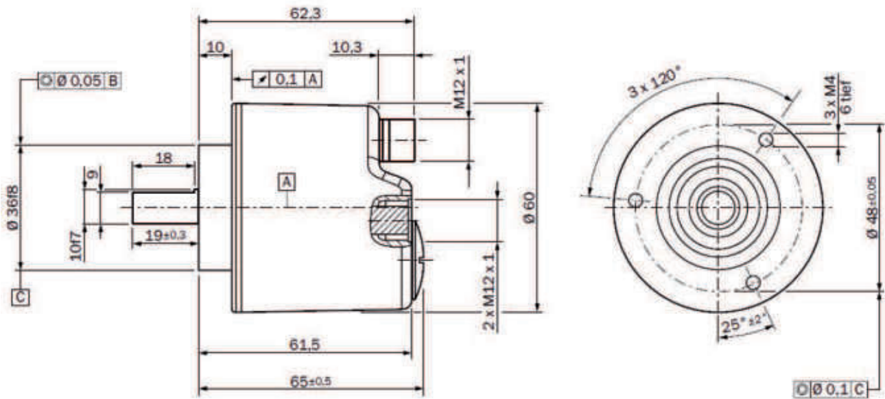
Dimensional drawing Solid shaft, face mount flange
