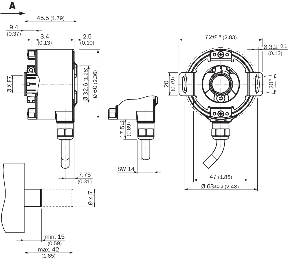
Customer-side Dimensions in mm (inch)
