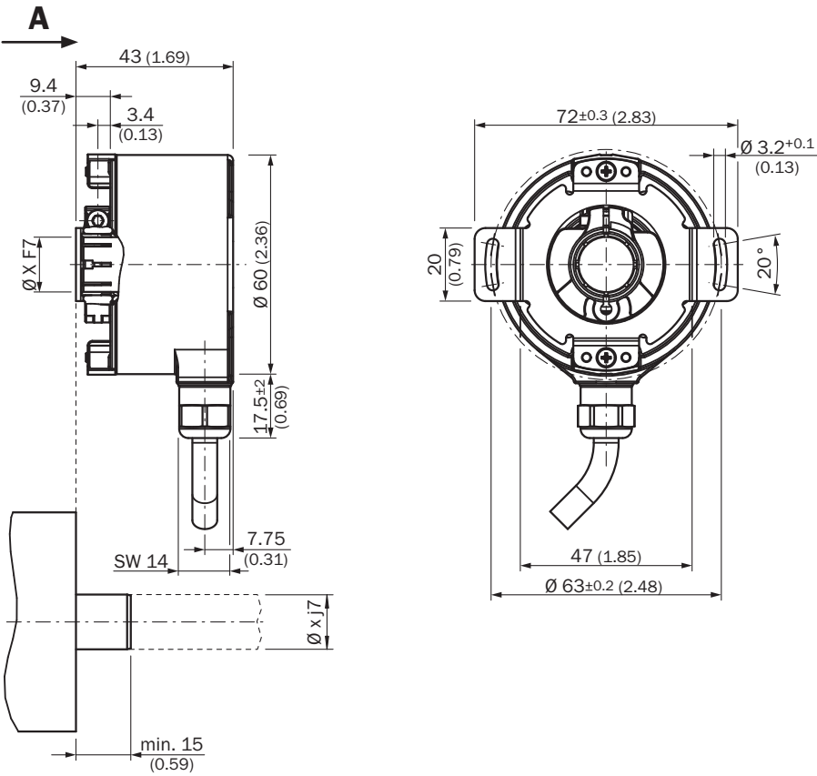
Customer-side Dimensions in mm (inch)
