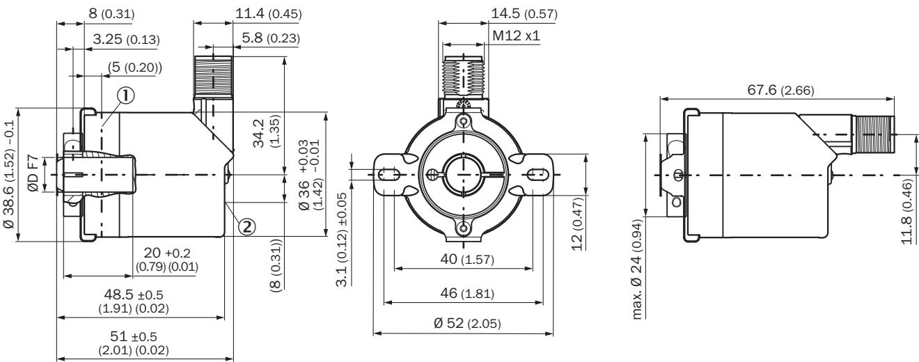
Dimensional drawing Blind hollow shaft, male connector
