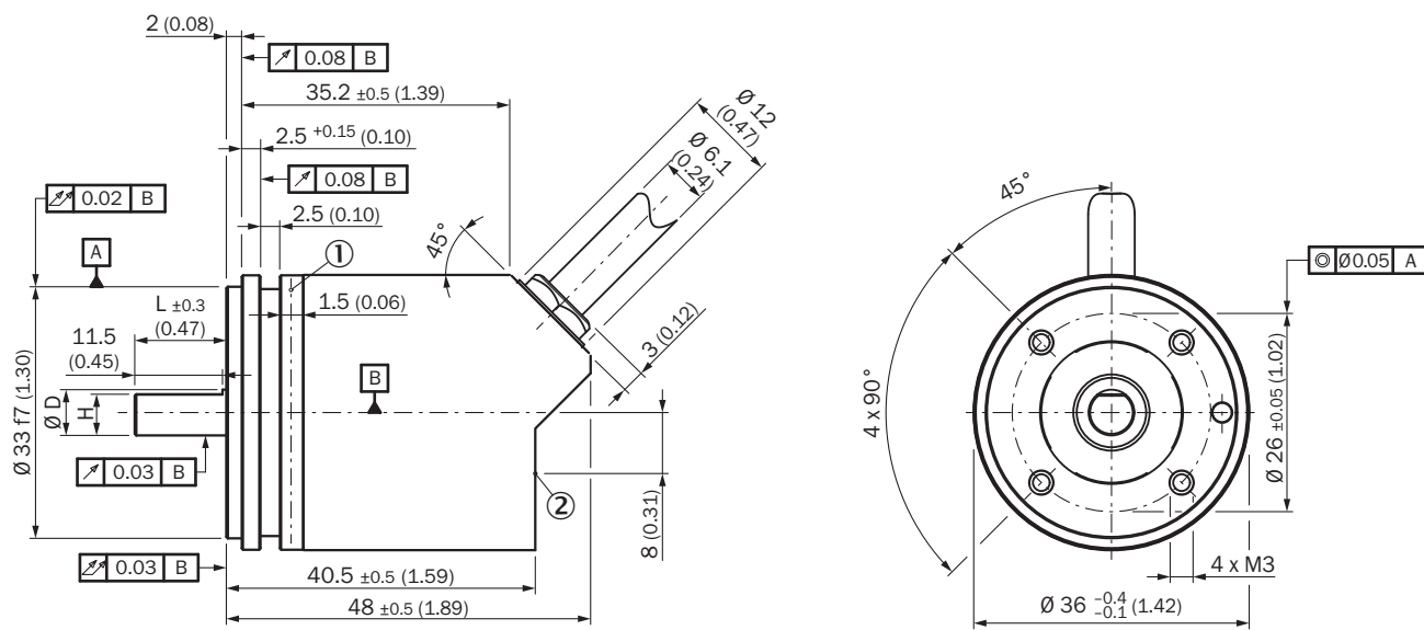
Dimensional drawing Solid shaft, servo flange, cable
