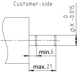
Dimensions in mm (inch)
