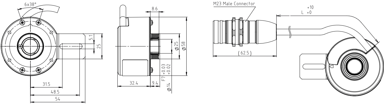
Dimensions in mm (inch)
