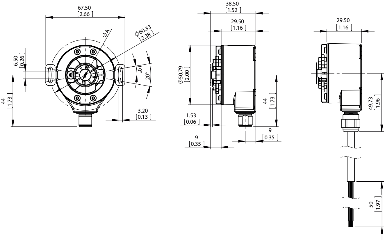
Dimensional drawing DFS21 through hollow shaft
