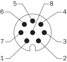
PIN assignment View of M12 male device connector on encoder
