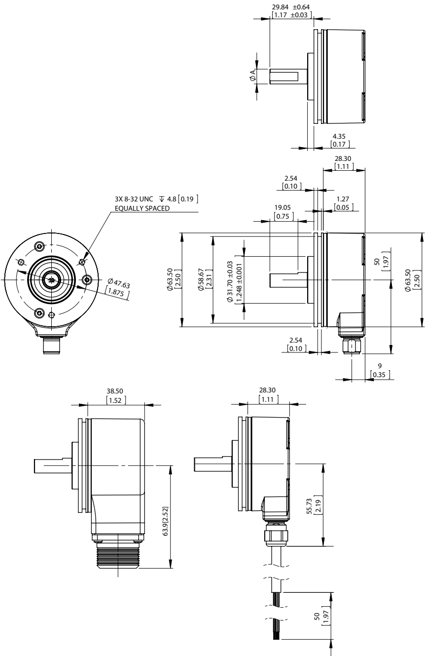
Dimensional drawing DFS25 servo flange mount, radial connector outlet M12 and MS, cable outlet
