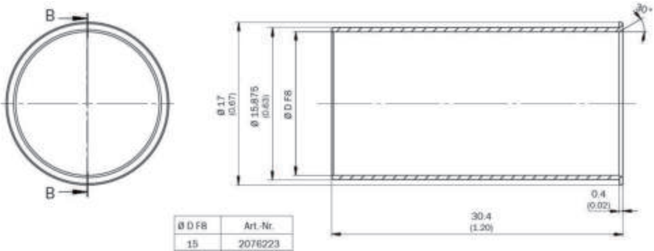
Dimensions in mm (inch)
