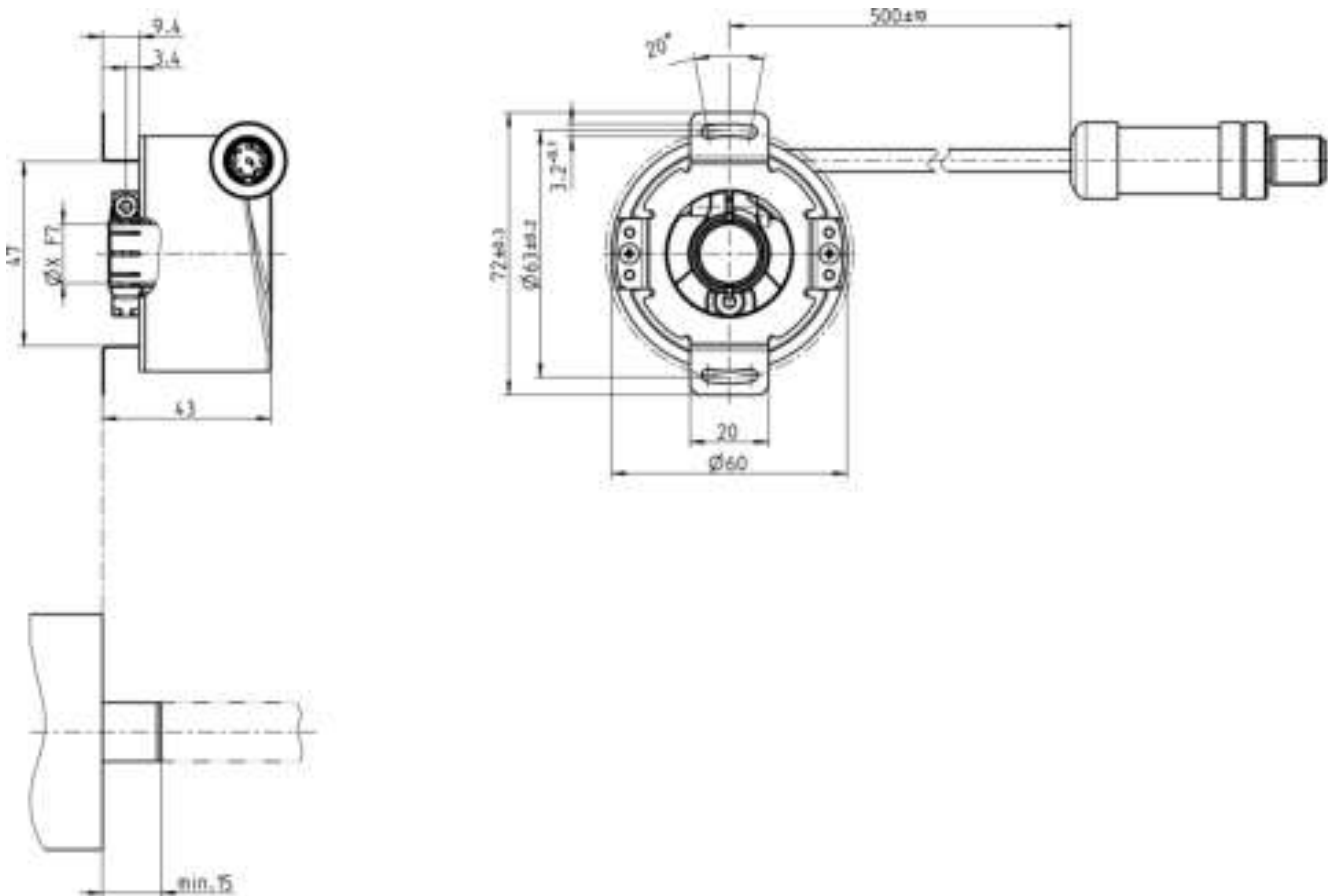
Dimensions in mm (inch) 6028369 Female Connector
