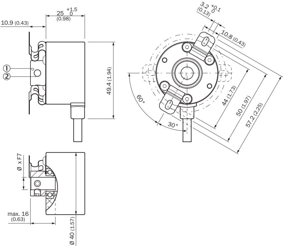
Dimensional drawing Blind hollow shaft
