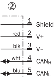
② male connector M12, 5-pin
