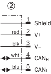
② male connector M12, 5-pin
