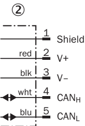
2 Connector M12, 5-pin, A-coded
