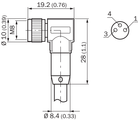
Dimensions in mm (inch)
