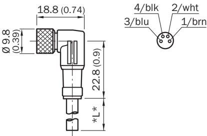
Dimensions in mm (inch)
