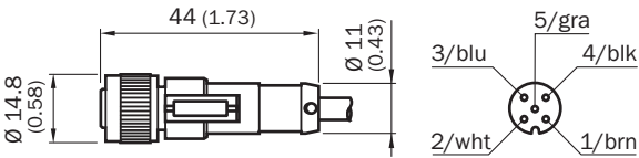
Dimensions in mm (inch)
